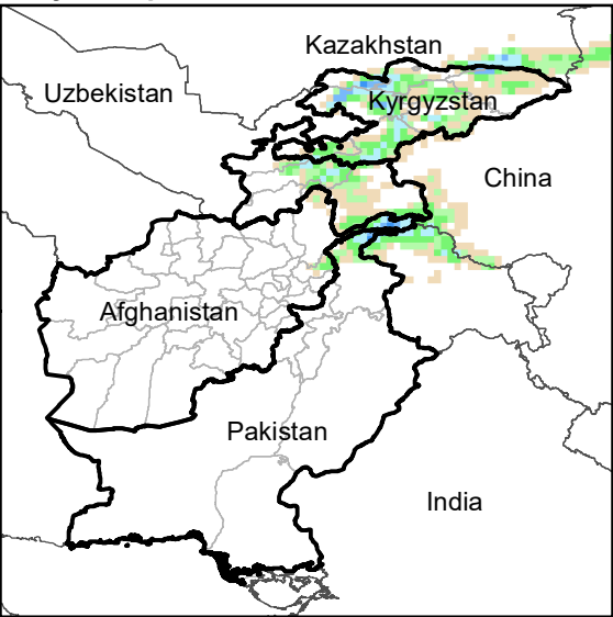
Daily Precip. Forecast for 31 Oct., 2020
