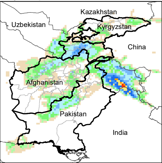
Daily Precip. Forecast for 11 Dec., 2020
