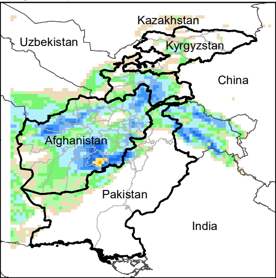
Daily Precip. Forecast for 10 Dec., 2020
