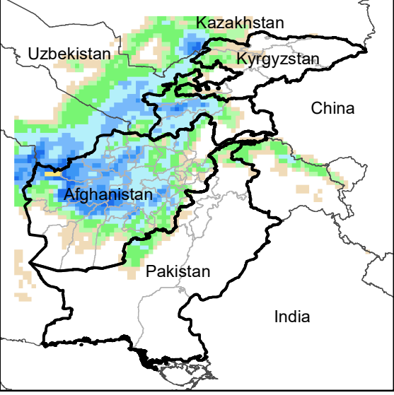
Daily Precip. Forecast for 26 Dec., 2020
