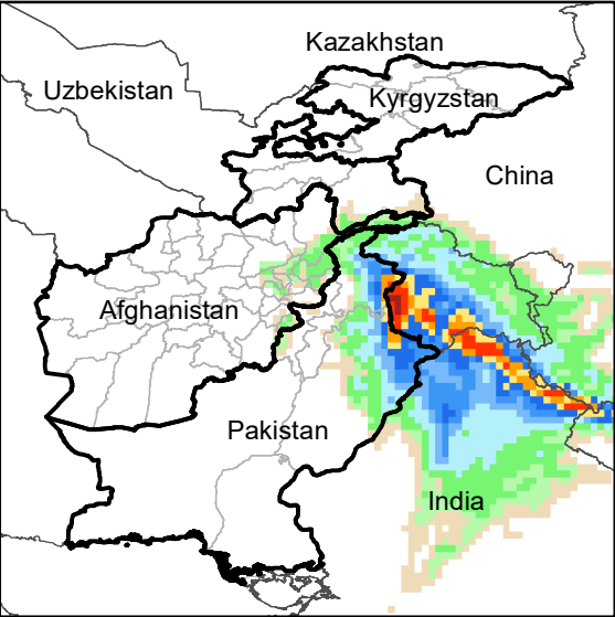
Daily Precip. Forecast for 5 Jan., 2021
