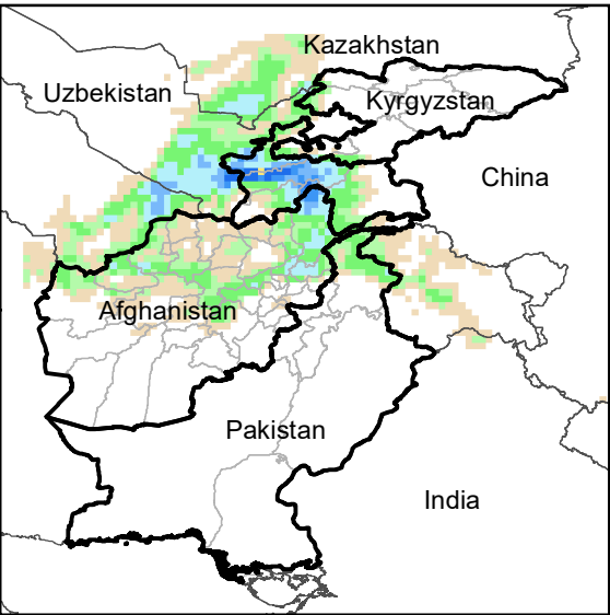
Daily Precip. Forecast for 3 Feb., 2021
