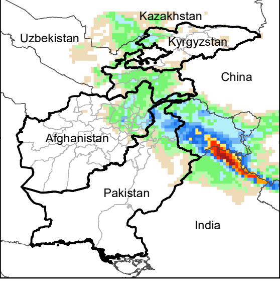
Daily Precip. Forecast for 7 Mar., 2021
