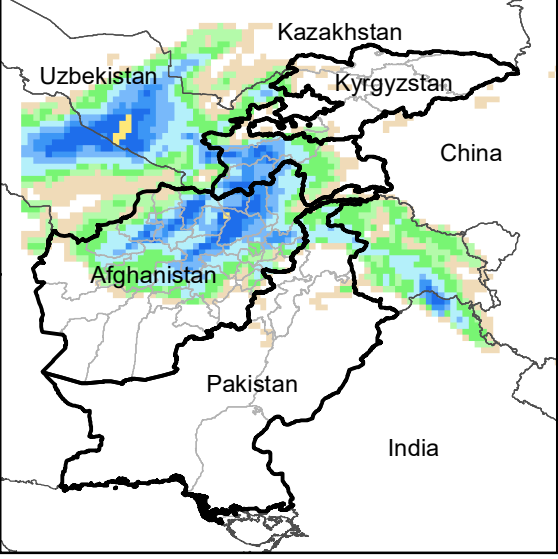
Daily Precip. Forecast for 6 Mar., 2021
