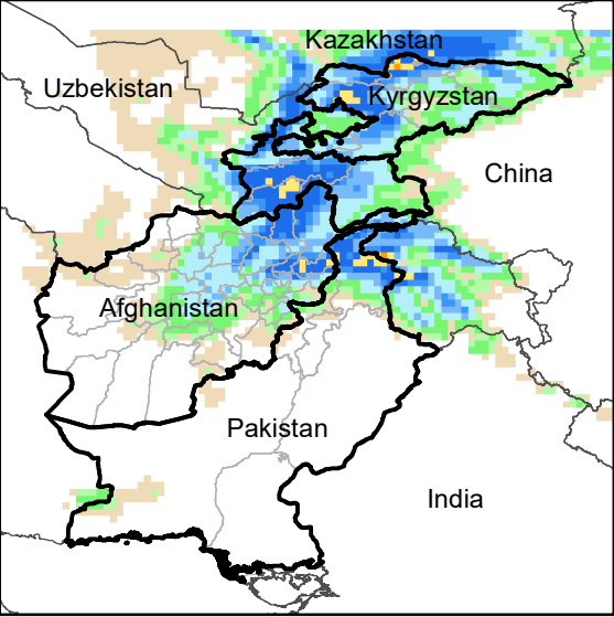
Daily Precip. Forecast for 14 Mar., 2021
