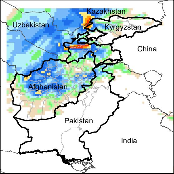
Daily Precip. Forecast for 13 Mar., 2021
