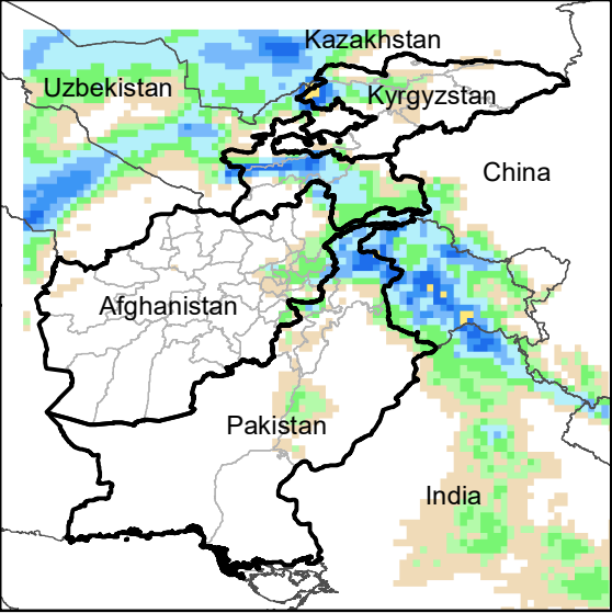
Daily Precip. Forecast for 12 Mar., 2021
