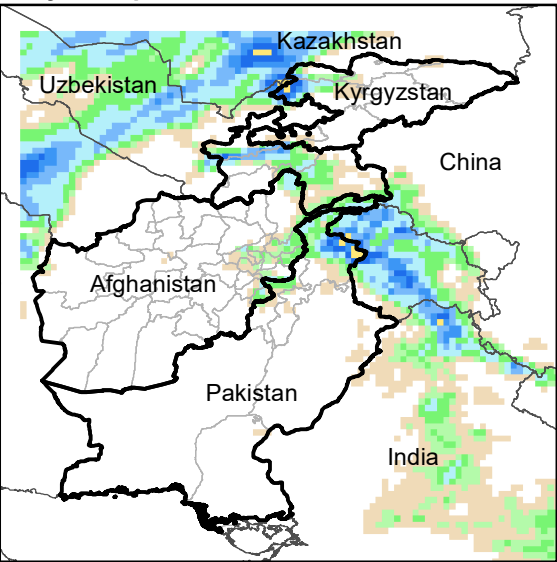
Daily Precip. Forecast for 15 Mar., 2021
