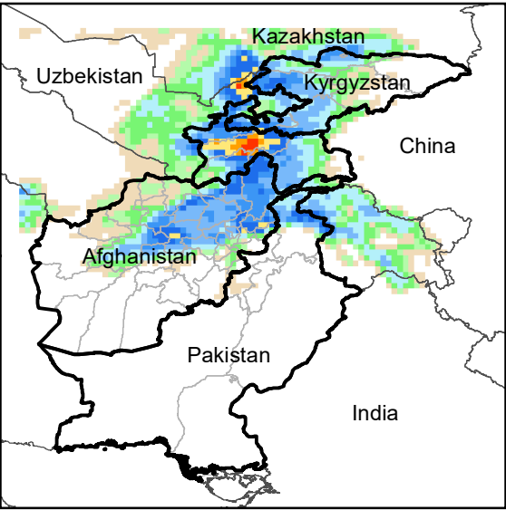
Daily Precip. Forecast for 4 Apr., 2021
