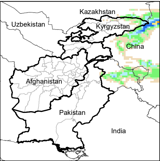
Daily Precip. Forecast for 5 Apr., 2021
