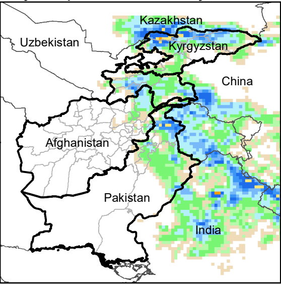
Daily Precip. Forecast for 12 May., 2021
