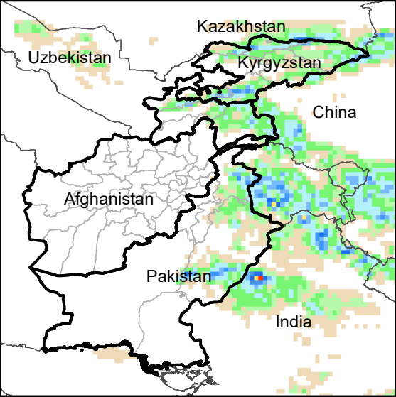
Daily Precip. Forecast for 3 Jun., 2021
