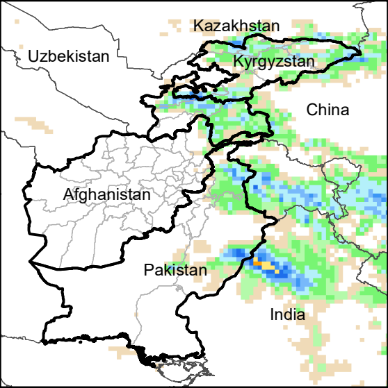
Daily Precip. Forecast for 2 Jun., 2021
