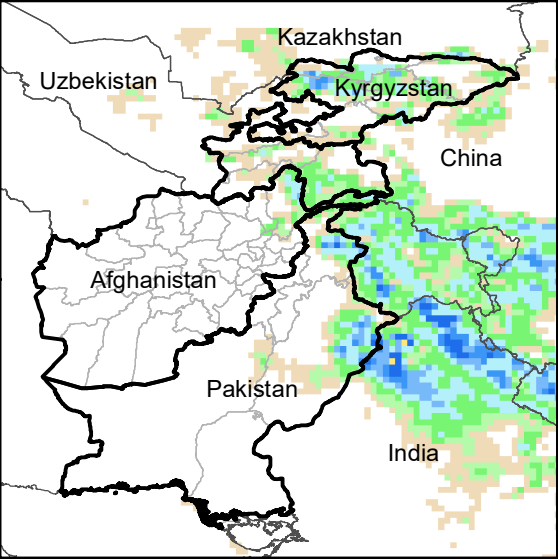
Daily Precip. Forecast for 1 Jun., 2021
