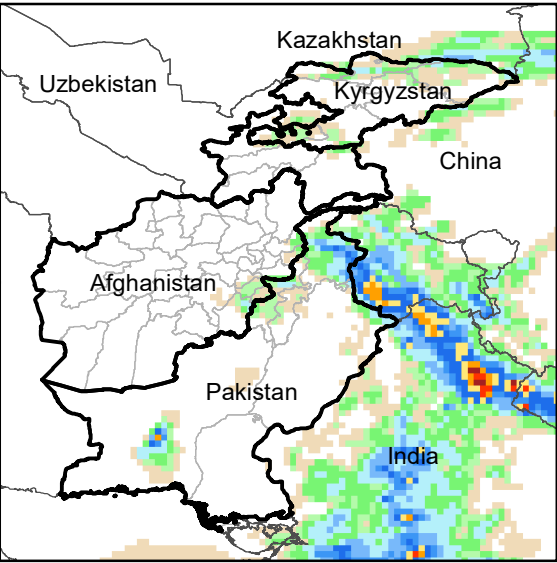
Daily Precip. Forecast for 11 Jul., 2021
