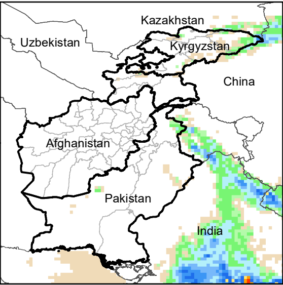
Daily Precip. Forecast for 10 Jul., 2021
