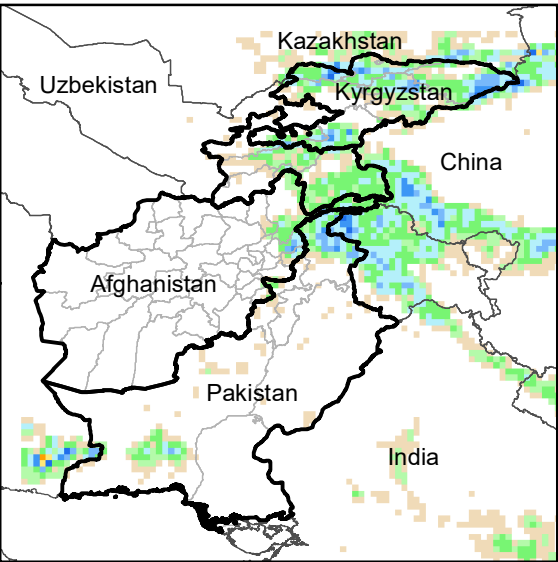
Daily Precip. Forecast for 9 Jul., 2021
