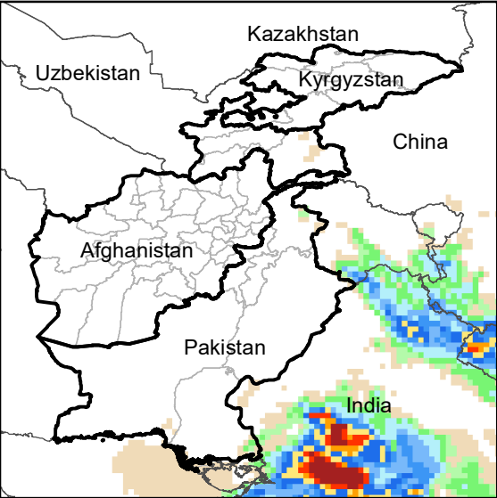
Daily Precip. Forecast for 28 Jul., 2021
