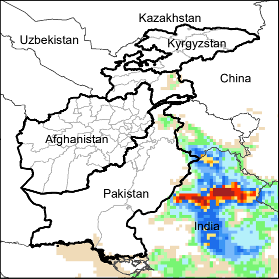
Daily Precip. Forecast for 26 Jul., 2021
