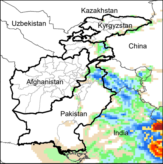
Daily Precip. Forecast for 27 Jul., 2021
