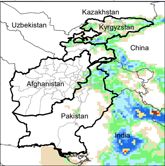
Daily Precip. Forecast for 7 Aug., 2021
