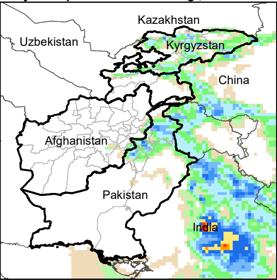
Daily Precip. Forecast for 5 Aug., 2021
