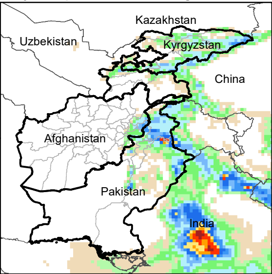
Daily Precip. Forecast for 6 Aug., 2021
