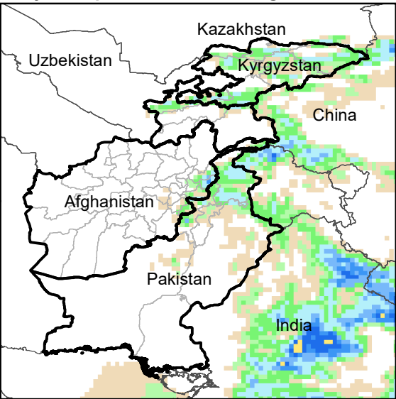
Daily Precip. Forecast for 10 Aug., 2021
