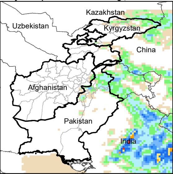
Daily Precip. Forecast for 9 Aug., 2021
