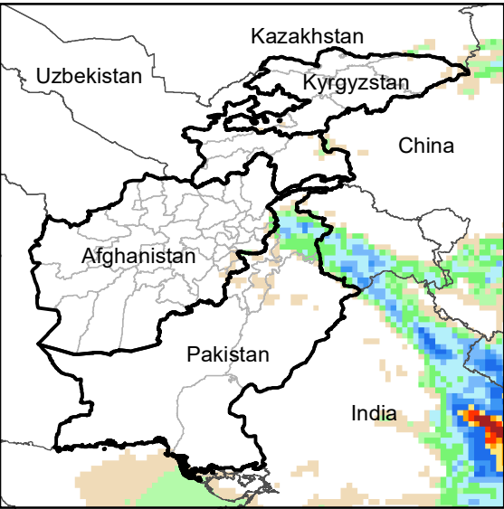
Daily Precip. Forecast for 11 Aug., 2021
