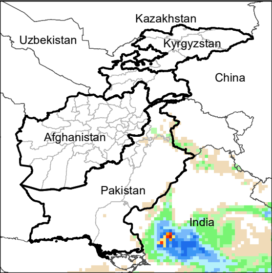
Daily Precip. Forecast for 18 Sep., 2021
