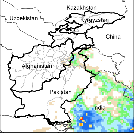
Daily Precip. Forecast for 19 Sep., 2021
