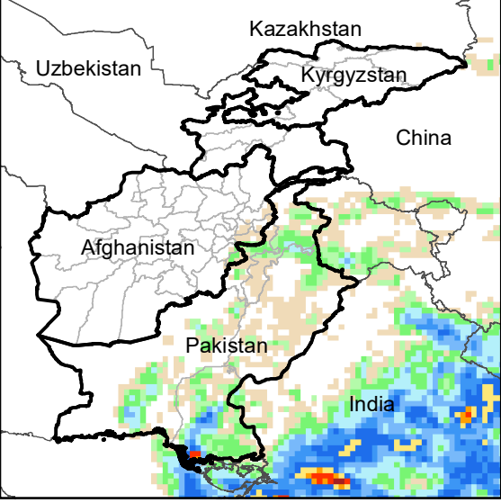
Daily Precip. Forecast for 24 Sep., 2021
