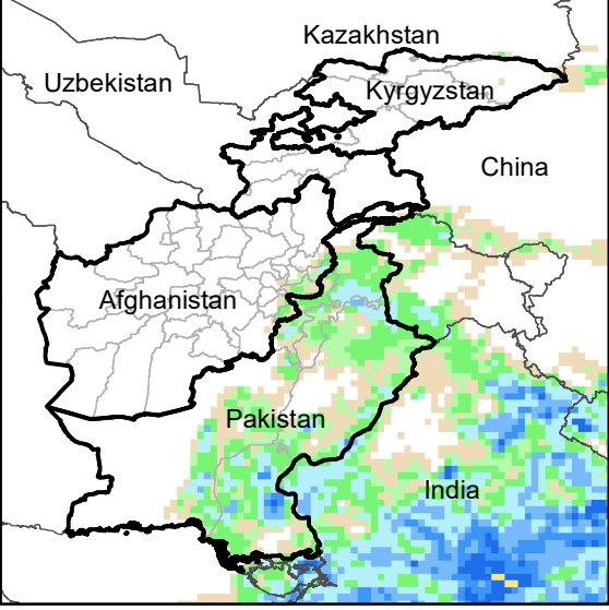
Daily Precip. Forecast for 23 Sep., 2021
