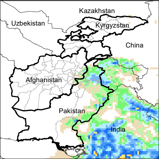
Daily Precip. Forecast for 21 Sep., 2021
