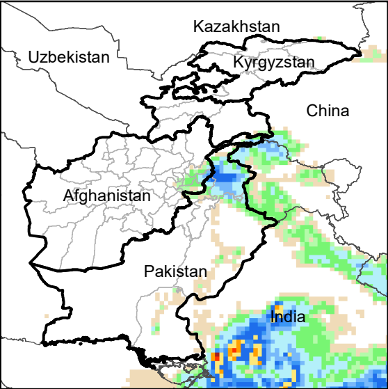
Daily Precip. Forecast for 20 Sep., 2021
