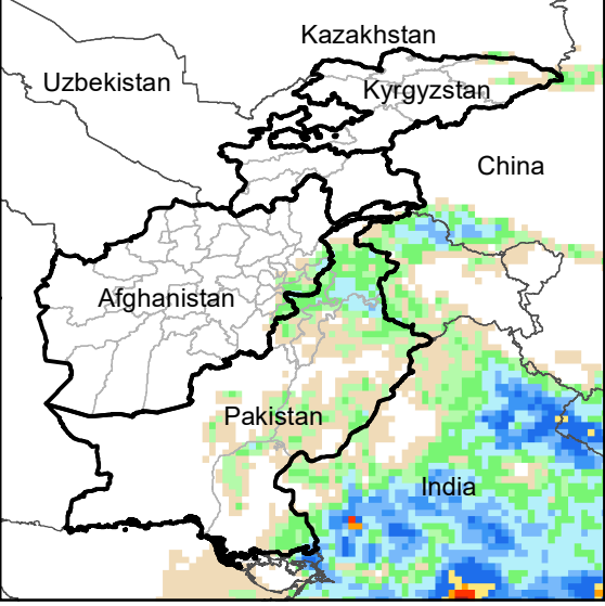
Daily Precip. Forecast for 22 Sep., 2021
