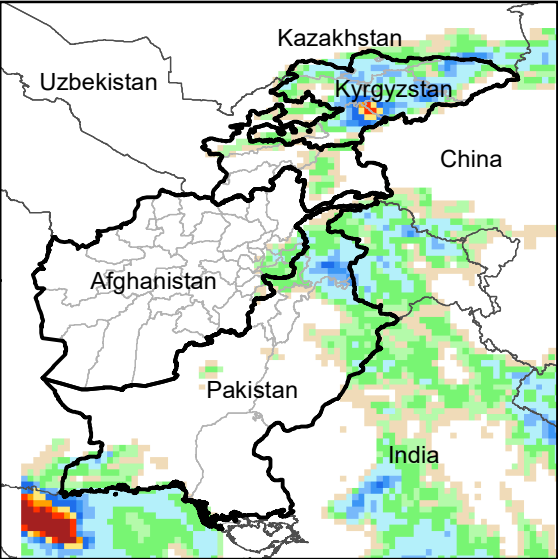
Daily Precip. Forecast for 5 Oct., 2021
