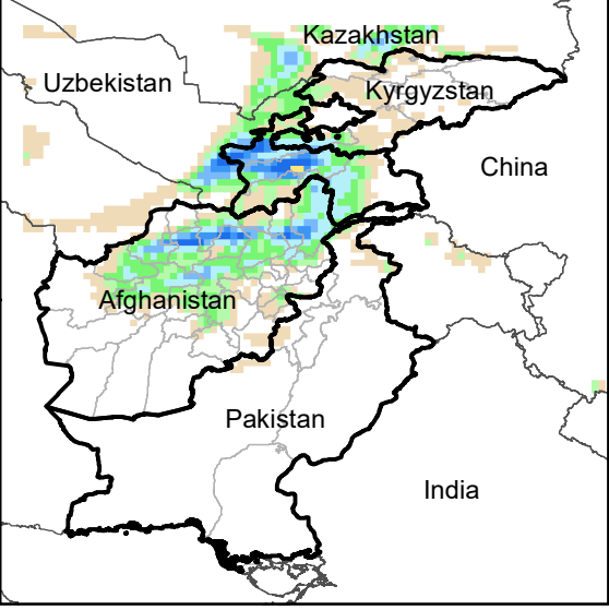
Daily Precip. Forecast for 22 Dec., 2021
