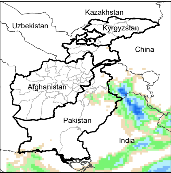
Daily Precip. Forecast for 28 Dec., 2021
