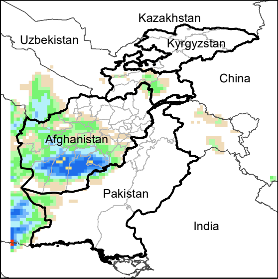
Daily Precip. Forecast for 31 Dec., 2021
