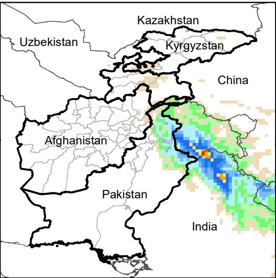
Daily Precip. Forecast for 26 Jan., 2022
