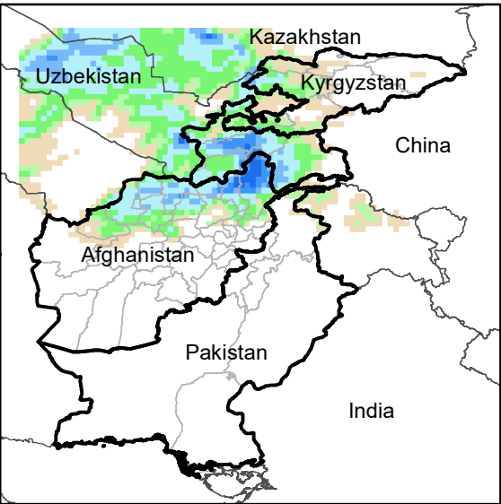
Daily Precip. Forecast for 31 Jan., 2022
