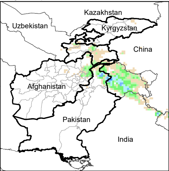
Daily Precip. Forecast for 3 Feb., 2022
