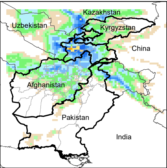
Daily Precip. Forecast for 9 Feb., 2022
