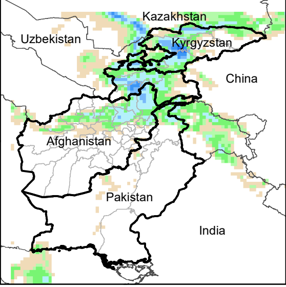
Daily Precip. Forecast for 14 Feb., 2022
