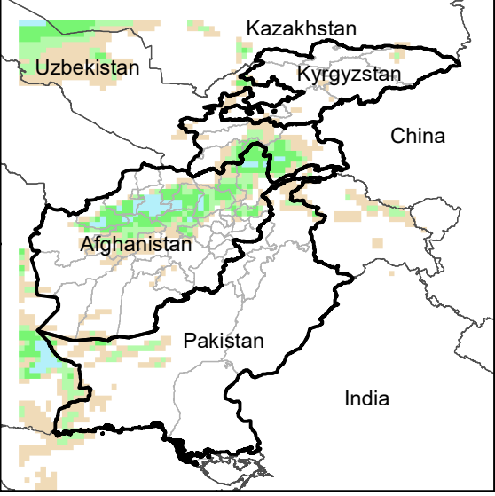
Daily Precip. Forecast for 13 Feb., 2022
