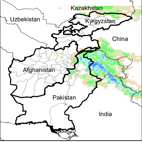
Daily Precip. Forecast for 15 Feb., 2022
