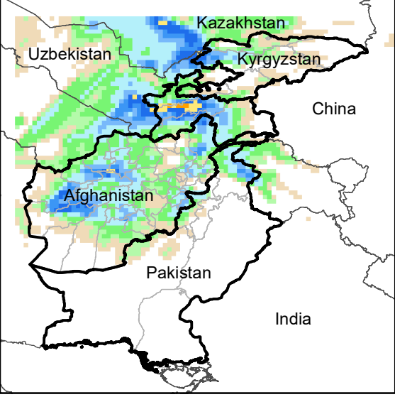
Daily Precip. Forecast for 5 Mar., 2022
