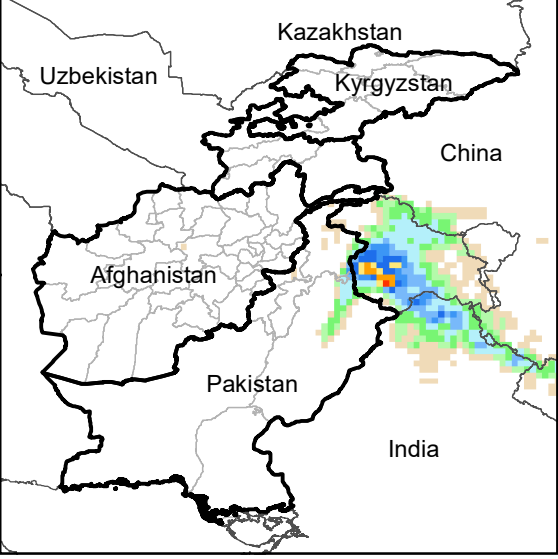
Daily Precip. Forecast for 3 Mar., 2022
