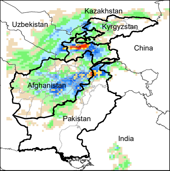
Daily Precip. Forecast for 8 Mar., 2022
