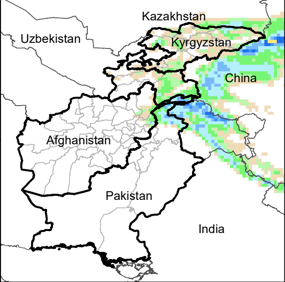
Daily Precip. Forecast for 20 Mar., 2022
