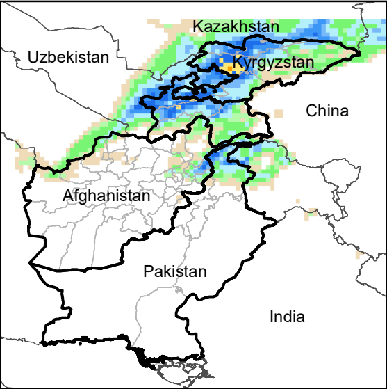
Daily Precip. Forecast for 21 Mar., 2022
