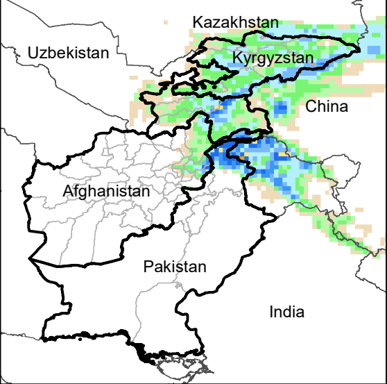
Daily Precip. Forecast for 19 Mar., 2022
