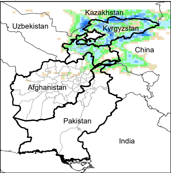
Daily Precip. Forecast for 1 Apr., 2022
