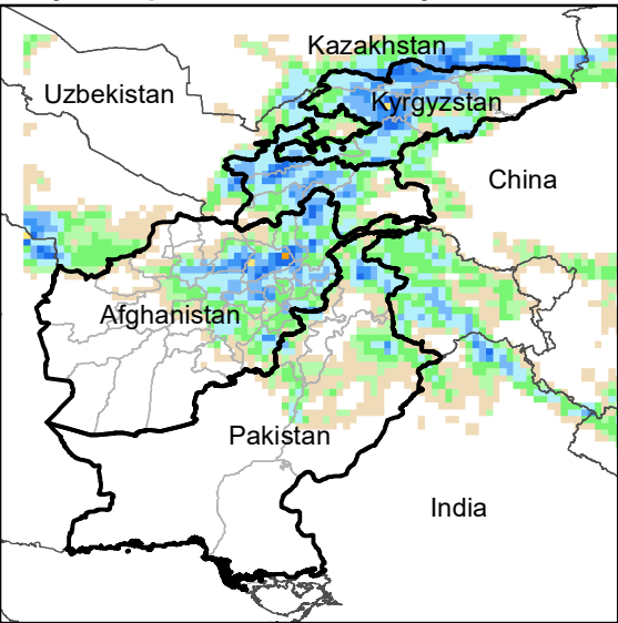
Daily Precip. Forecast for 7 May., 2022
