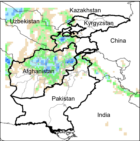
Daily Precip. Forecast for 5 May., 2022
