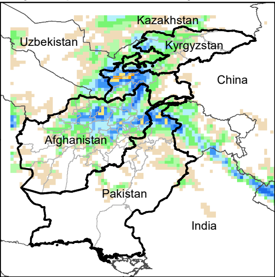
Daily Precip. Forecast for 6 May., 2022
