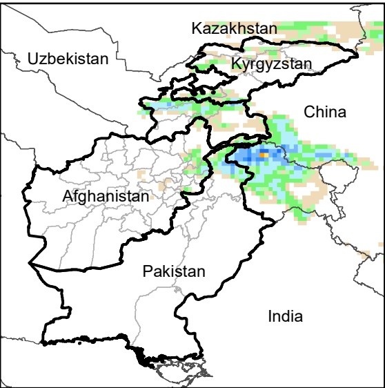
Daily Precip. Forecast for 4 Jun., 2022
