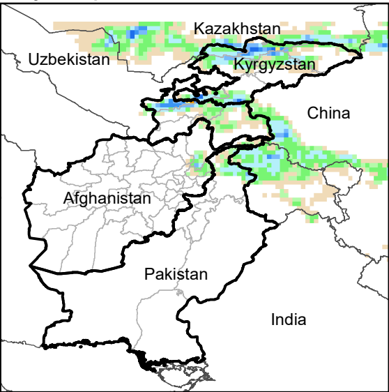
Daily Precip. Forecast for 5 Jun., 2022
