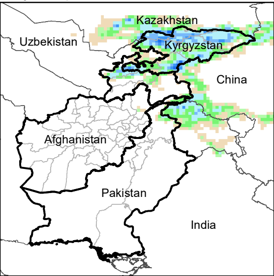
Daily Precip. Forecast for 6 Jun., 2022
