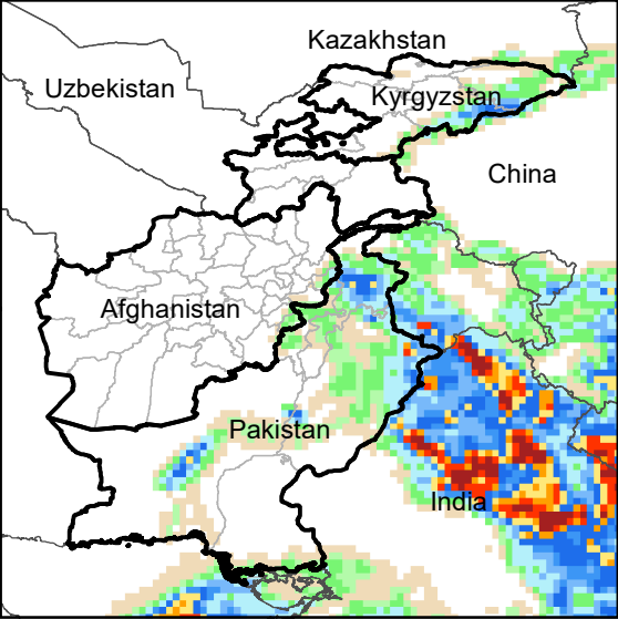
Daily Precip. Forecast for 9 Jul., 2022
