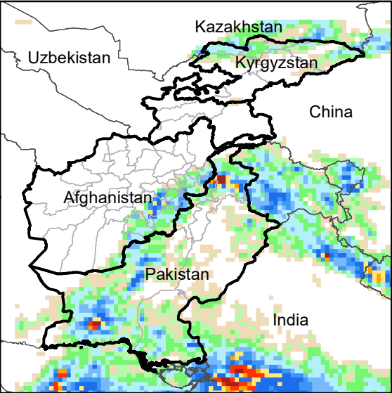
Daily Precip. Forecast for 8 Jul., 2022
