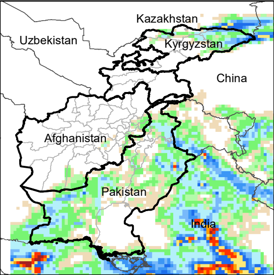
Daily Precip. Forecast for 10 Jul., 2022
