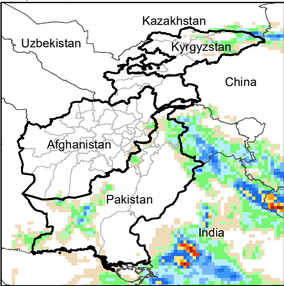
Daily Precip. Forecast for 22 Jul., 2022
