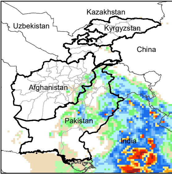
Daily Precip. Forecast for 23 Jul., 2022
