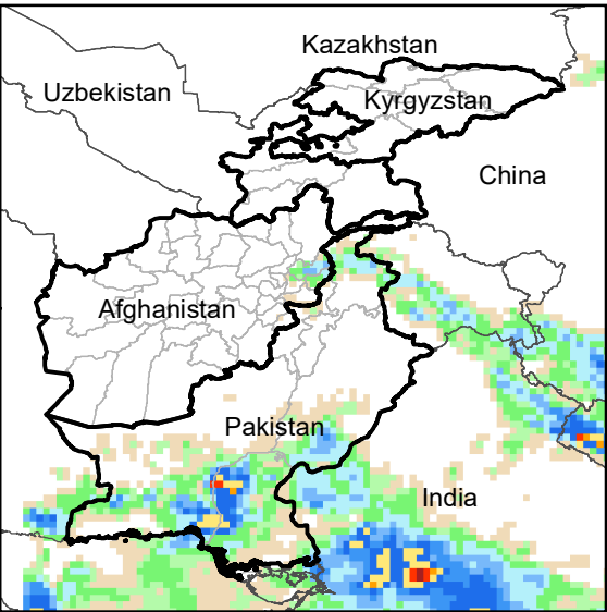
Daily Precip. Forecast for 21 Jul., 2022
