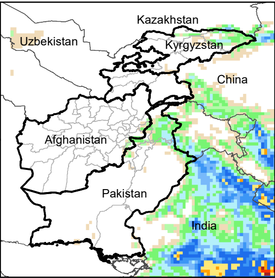
Daily Precip. Forecast for 7 Aug., 2022
