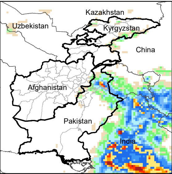
Daily Precip. Forecast for 8 Aug., 2022
