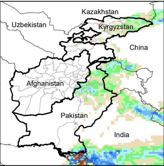
Daily Precip. Forecast for 12 Sep., 2022
