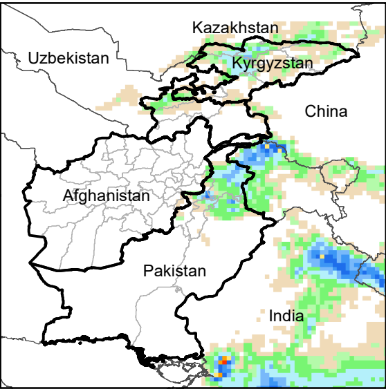
Daily Precip. Forecast for 11 Sep., 2022
