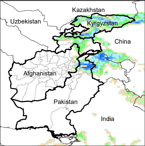
Daily Precip. Forecast for 4 Oct., 2022
