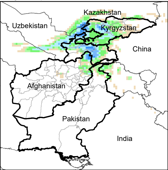
Daily Precip. Forecast for 27 Oct., 2022
