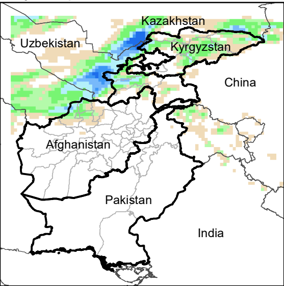
Daily Precip. Forecast for 28 Oct., 2022
