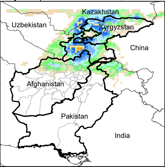
Daily Precip. Forecast for 26 Oct., 2022
