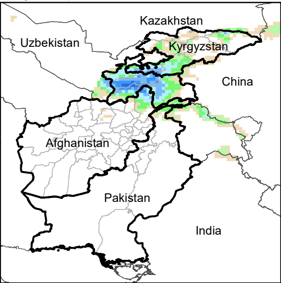
Daily Precip. Forecast for 5 Dec., 2022
