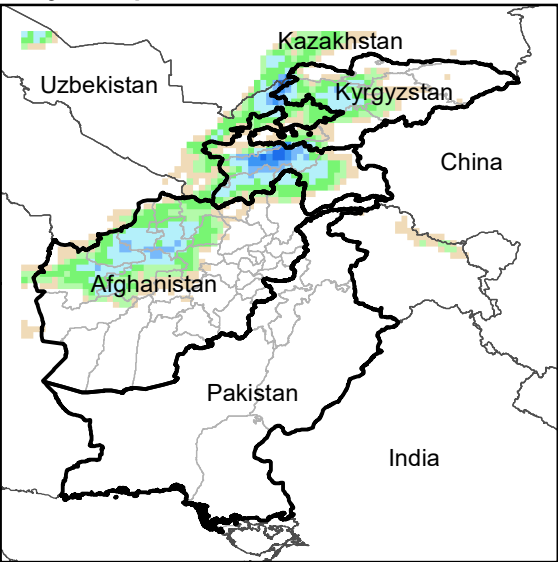
Daily Precip. Forecast for 10 Dec., 2022
