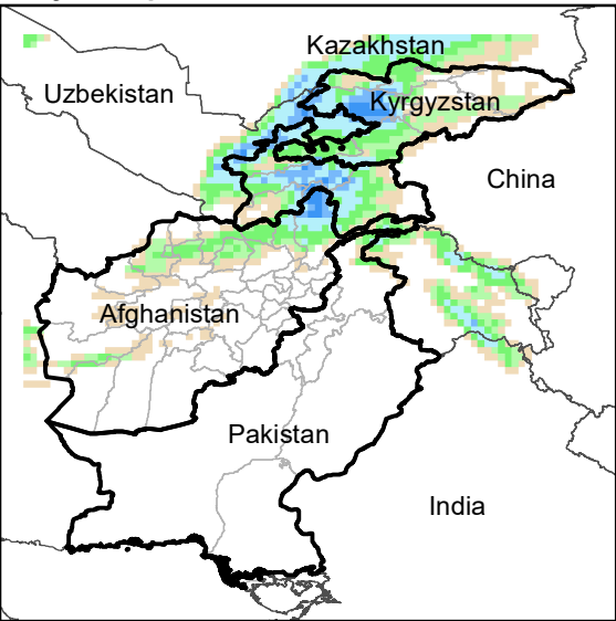
Daily Precip. Forecast for 11 Dec., 2022
