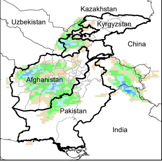
Daily Precip. Forecast for 29 Dec., 2022
