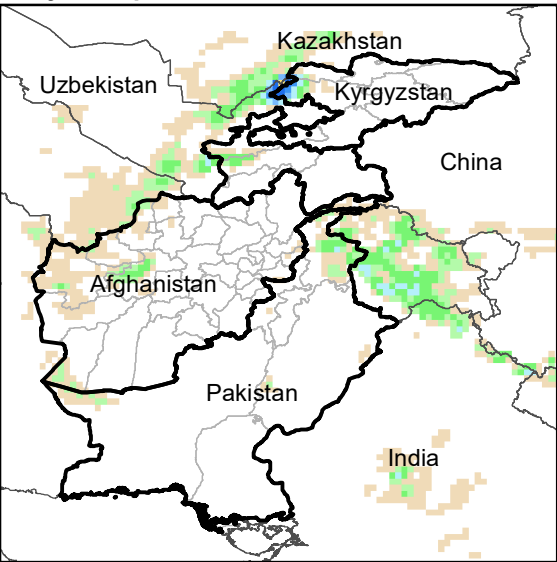
Daily Precip. Forecast for 8 Mar., 2023
