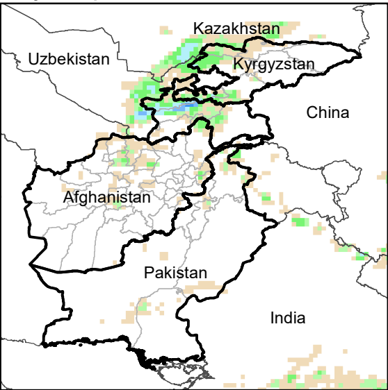
Daily Precip. Forecast for 9 Mar., 2023
