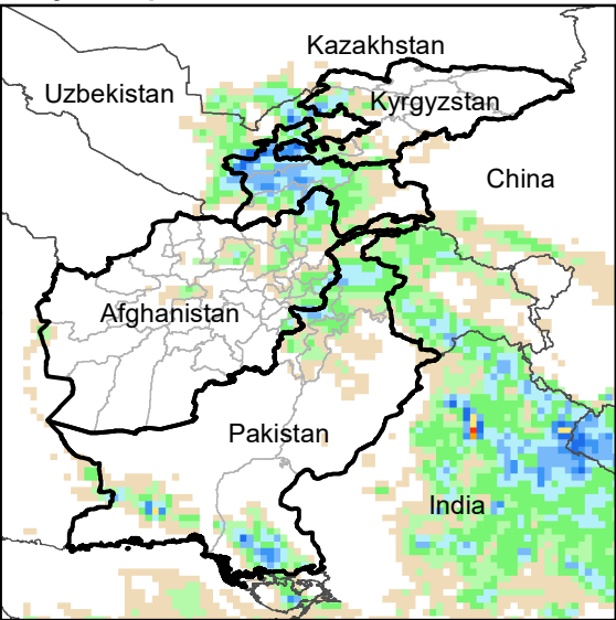
Daily Precip. Forecast for 23 Mar., 2023
