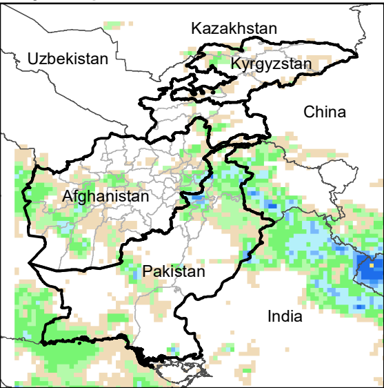
Daily Precip. Forecast for 24 Mar., 2023
