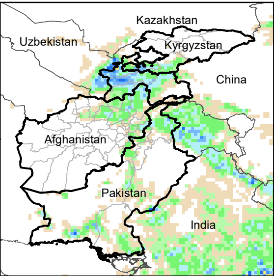
Daily Precip. Forecast for 22 Mar., 2023
