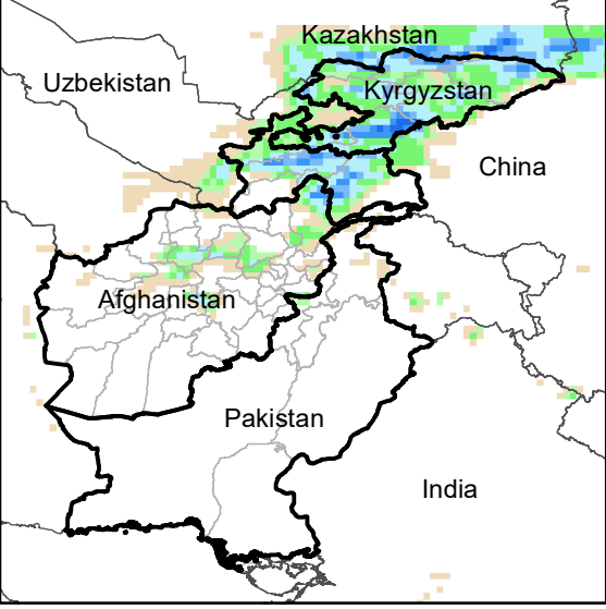
Daily Precip. Forecast for 8 Apr., 2023
