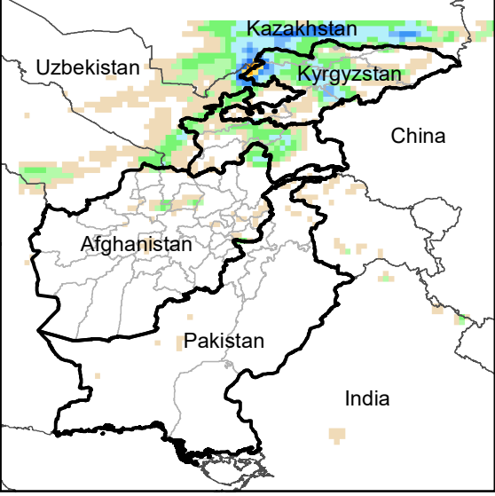
Daily Precip. Forecast for 7 Apr., 2023
