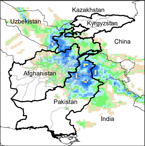
Daily Precip. Forecast for 3 Apr., 2023
