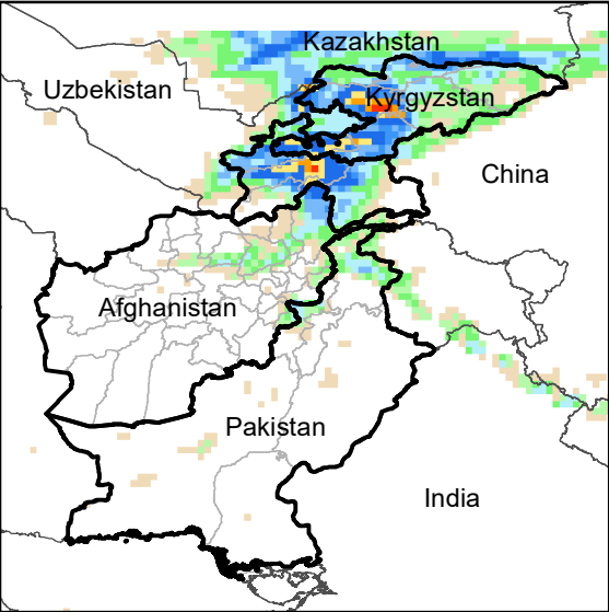
Daily Precip. Forecast for 13 Apr., 2023
