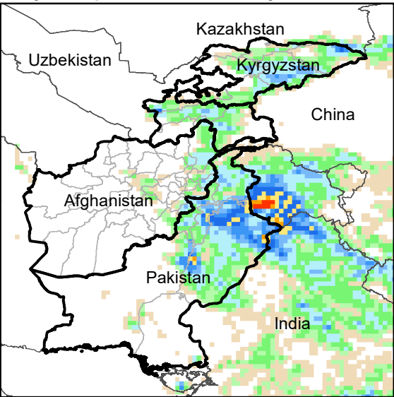
Daily Precip. Forecast for 5 May., 2023
