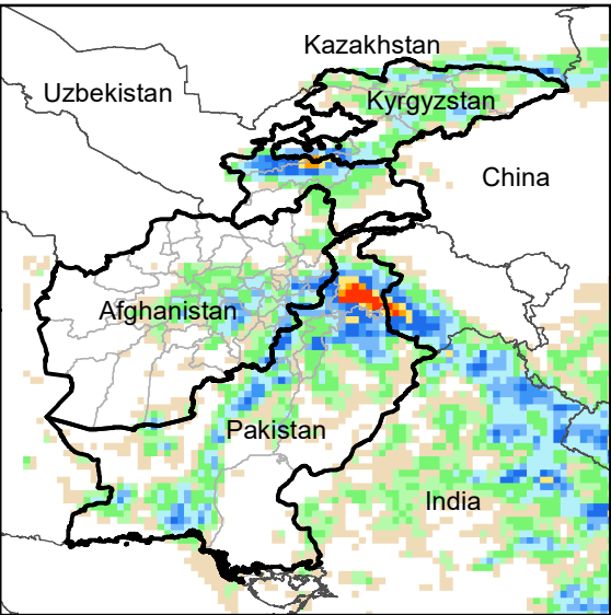
Daily Precip. Forecast for 4 May., 2023
