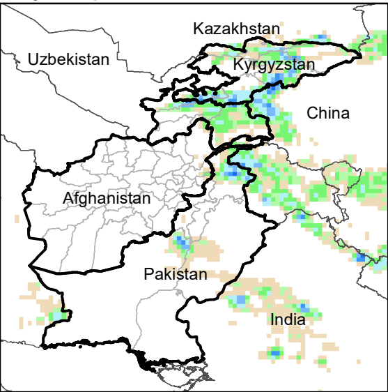
Daily Precip. Forecast for 8 Jun., 2023
