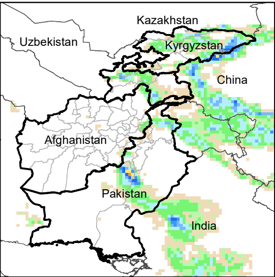
Daily Precip. Forecast for 6 Jun., 2023
