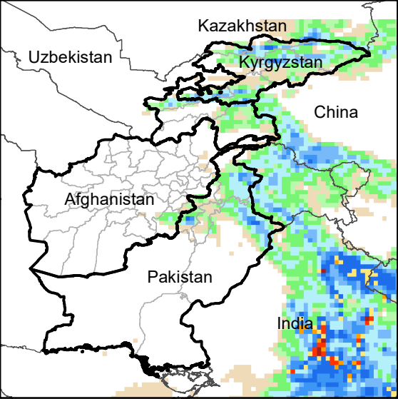
Daily Precip. Forecast for 4 Jul., 2023
